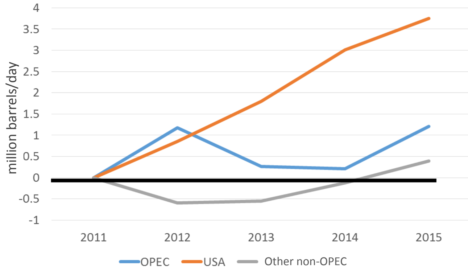
Cumulative crude production change since 2011
