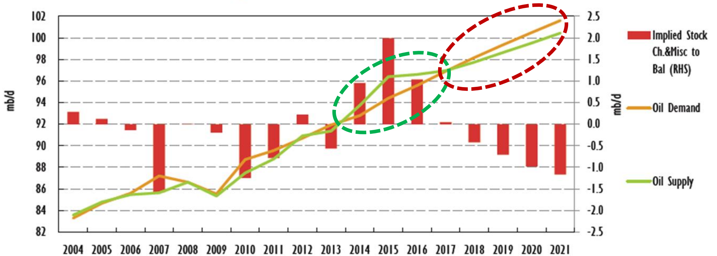
Figure ES 1 Global balance base case
